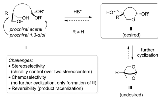
Scheme 1. Reaction design.
